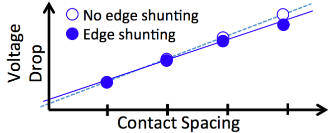
Fig. 6. Rollover effect in the TLM method leading to an overestimation of the y-intercept value
