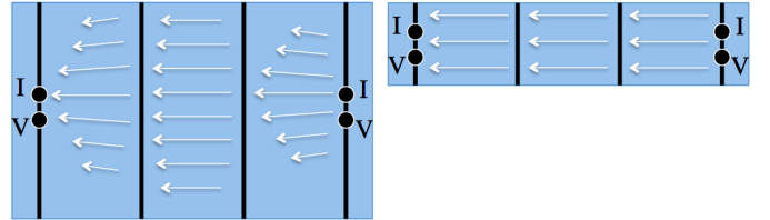
Fig. 7. Schematic depicting nonuniform current flow in a wide strip and uniform current flow in a narrow strip
