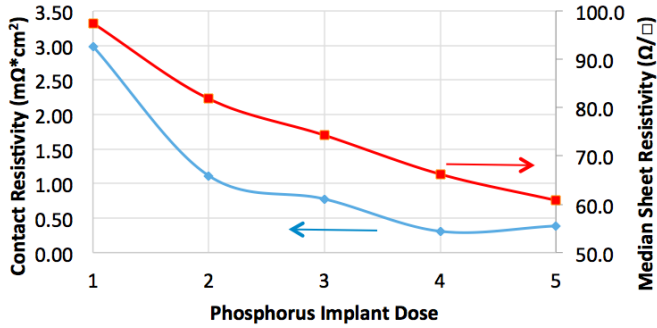
Fig. 2. Effective contact resistivity and sheet resistivity vs P implant dose as measured with the ContactSpot
