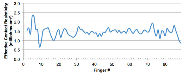
Fig. 4. Effective contact resistivity measurements across a full strip as measured with the ContactSpot
