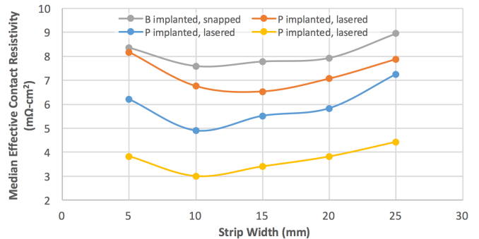
Fig. 5. Effective contact resistivity vs strip width for 4 different implanted layers
